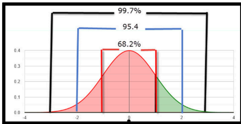
Exhibit 3.43—Empirical Rule of Standard Deviation.
