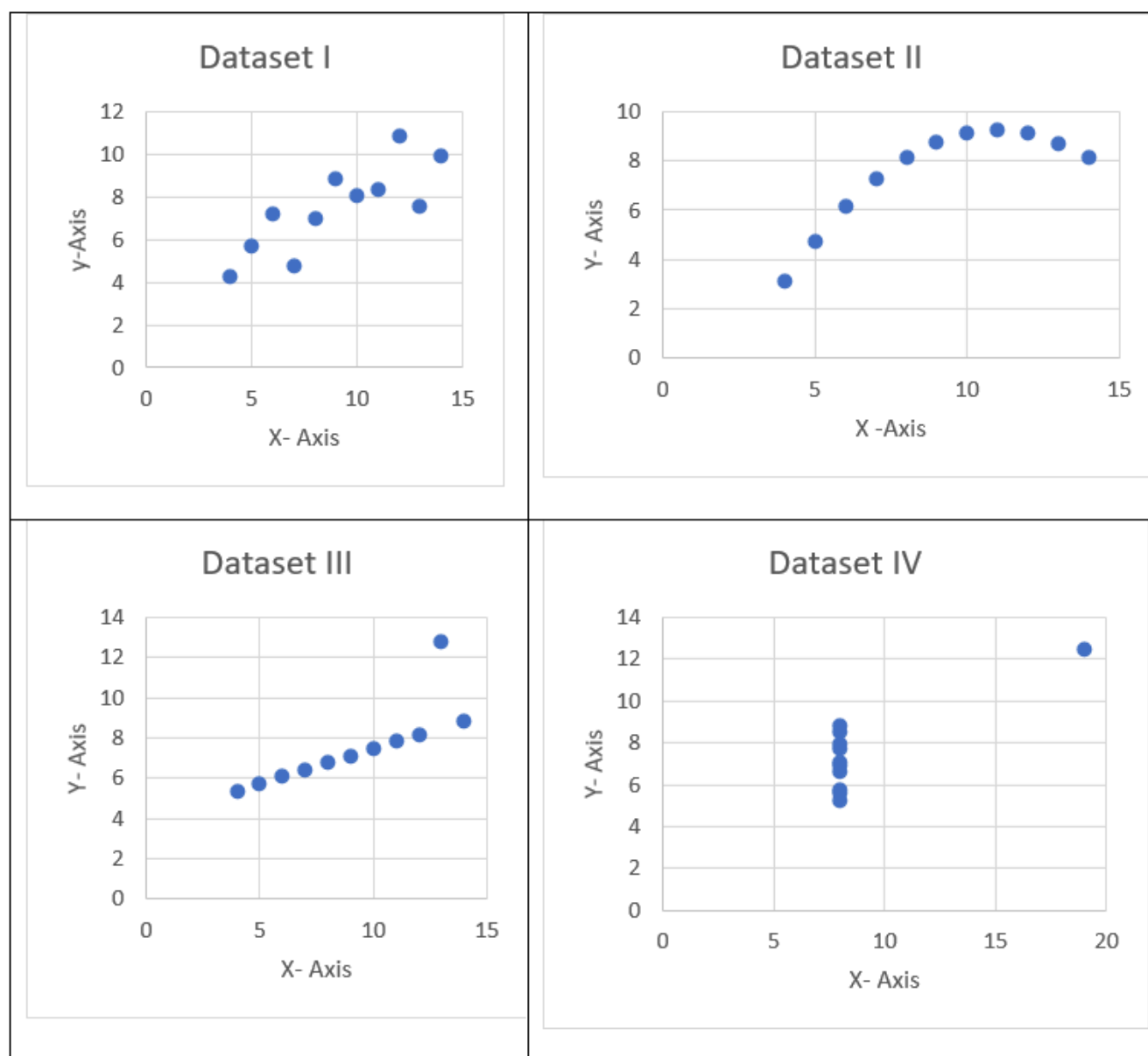
Figure 3.3—Scatterplots of the Anscombe's Quartet
